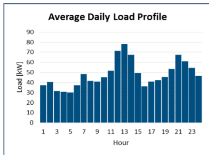
Figure 2: Example of a safari lodge's average daily load profile. 3
